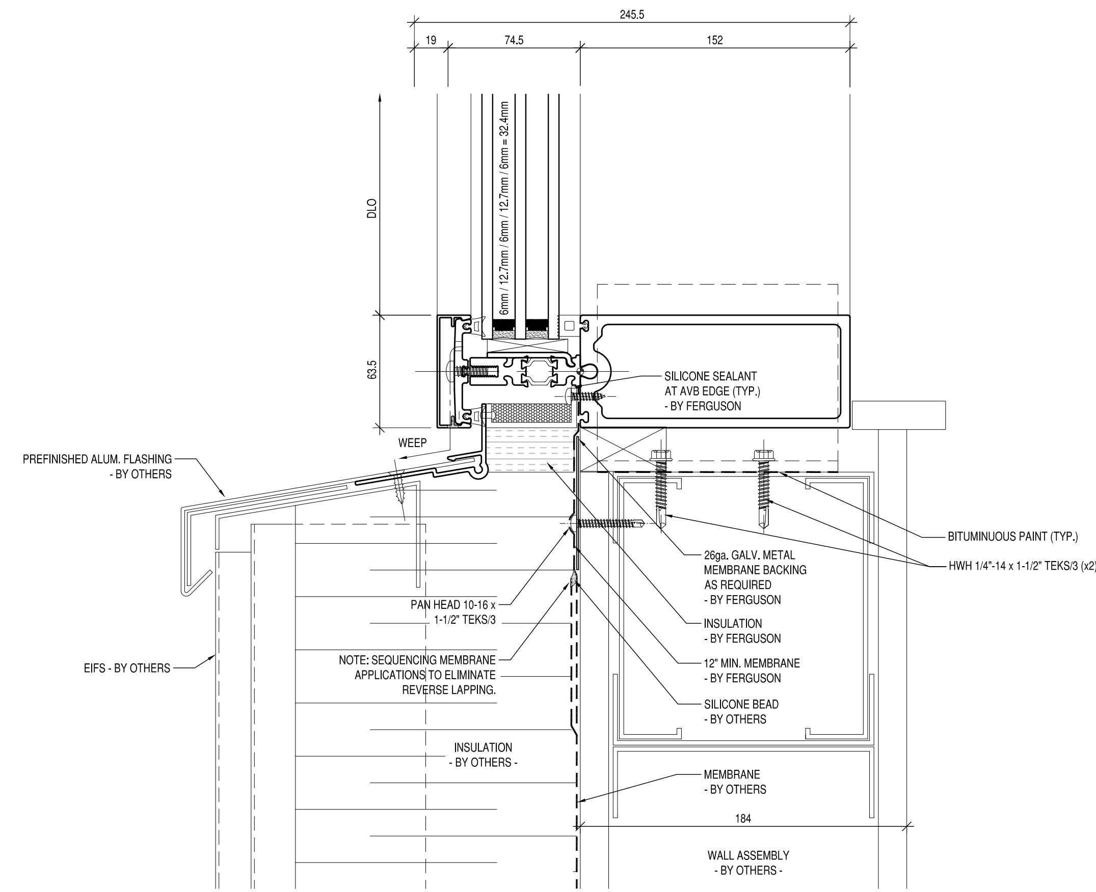
SILL SECTION
