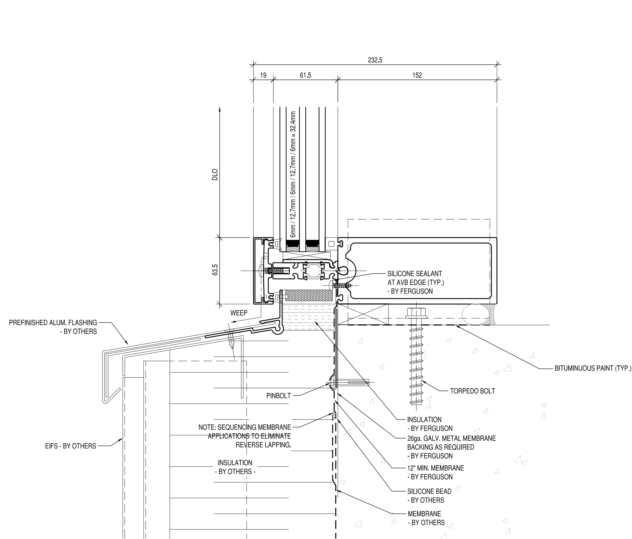
SILL SECTION
